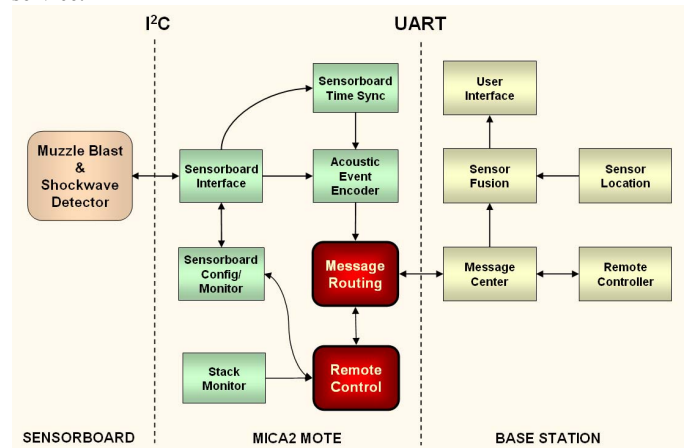
Figure 4. Software Architecture
