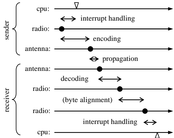
Figure 2. The timing of the transmission of an idealized point in the software (cpu), hardware (radio chip) and physical (antenna) layers of the sender and the receiver.
