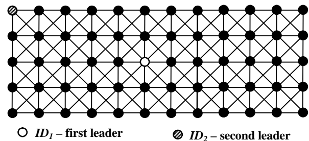
Figure 8. The layout and links of the experimental setup. Each node can only communicate with its (at most 8) neighbors.
