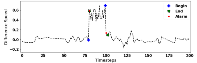
Figure 7. Detection of anomaly through CUSUM algorithm
