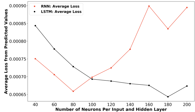
Figure 1. Average loss from predicted speed values by RNN and LSTM for different number of neurons
