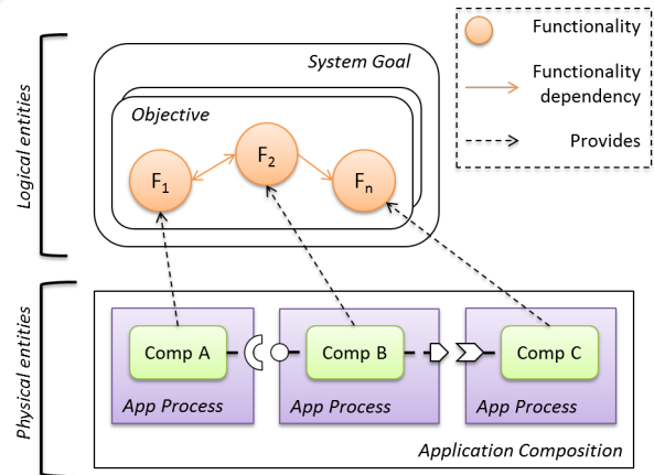
Figure 3: Example of a Goal-based Description of an Application.
