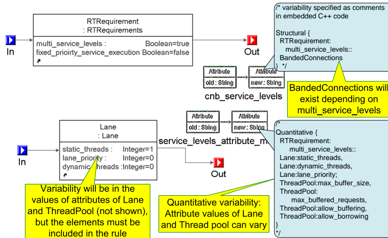
Fig. 5: Templated Transformation Rule in QoS Configuration Case Study.
